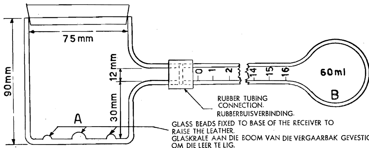
FIGURE 1.—Kubelka apparatus for the determination of water absorption.
