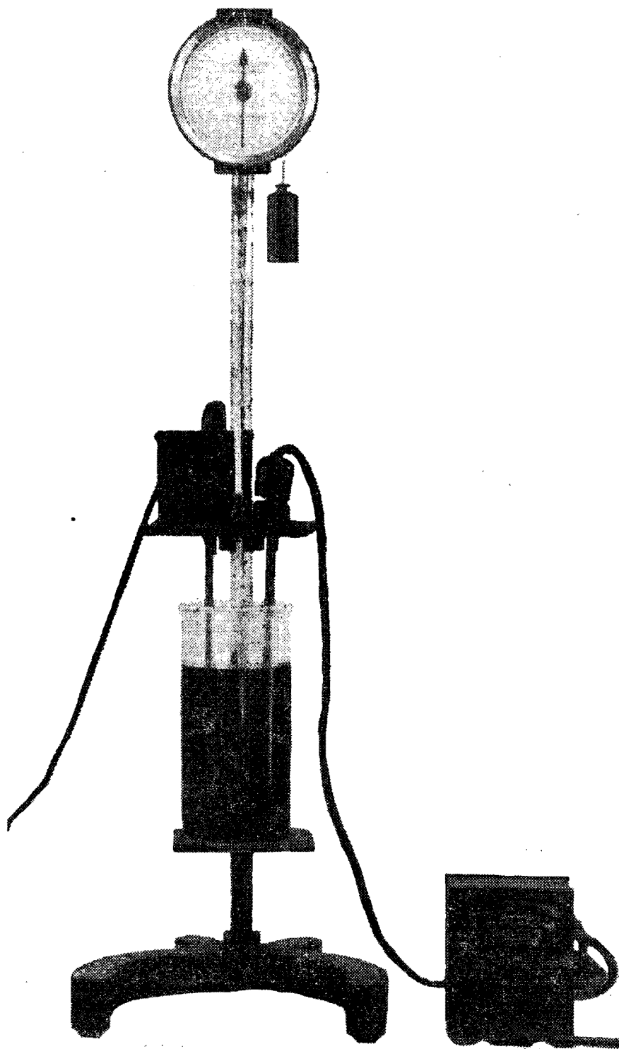
FIGURE 3.—Shrinkage test apparatus.
