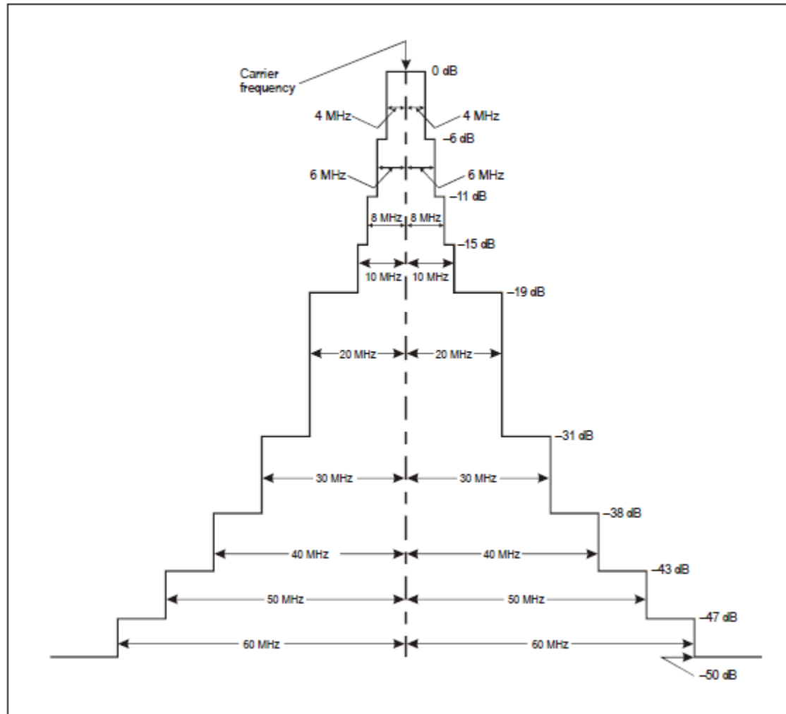
1.2 Figure 1-2: Required spectrum limits for interrogator transmitter (regulation 42)
