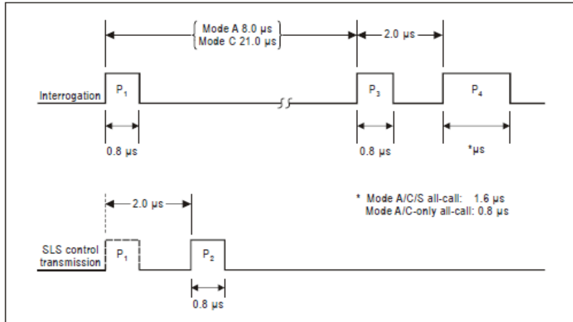
1.3 Figure 1-3: : Intermode interrogation pulse sequence (regulation 42)
