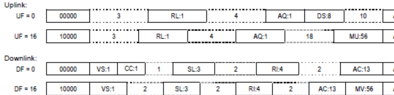
Figure 4-1: Surveillance and Communication formats used by ACAS
