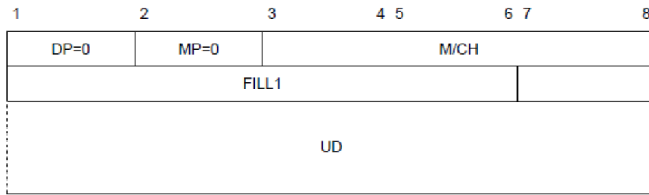
Figure 5-21. SHORT FORM MSP packet
