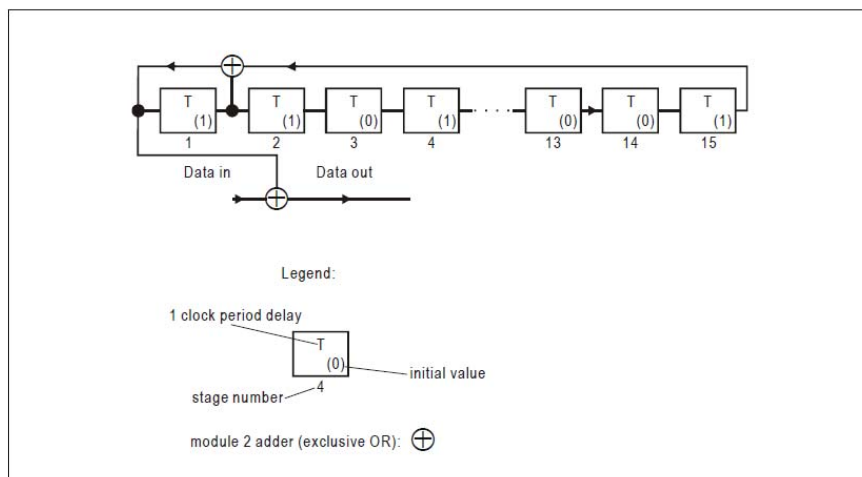
Figure 6-2. PN-generator for bit scrambling sequence
