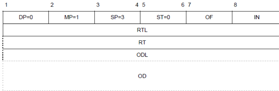
Figure 5-19. ROUTE packet
