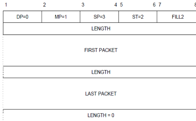
Figure 5-20. MULTIPLEX packet
