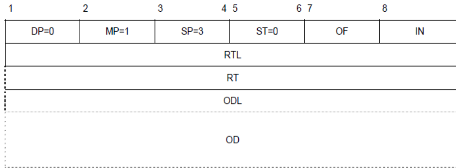
Figure 5-19. ROUTE packet
