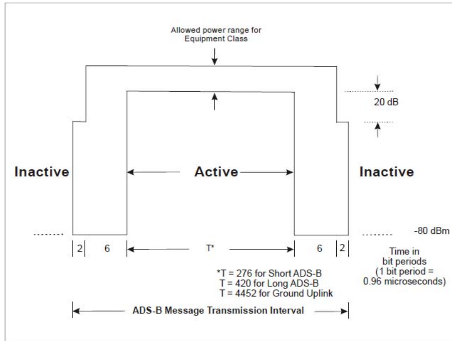
Figure 12-2. Time/amplitude profile of UAT message transmission
