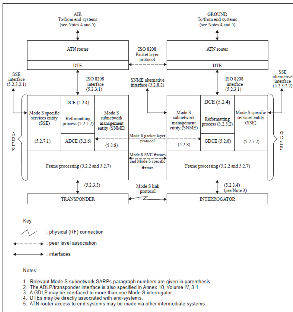
Functional elements of the Mode S subnetwork
