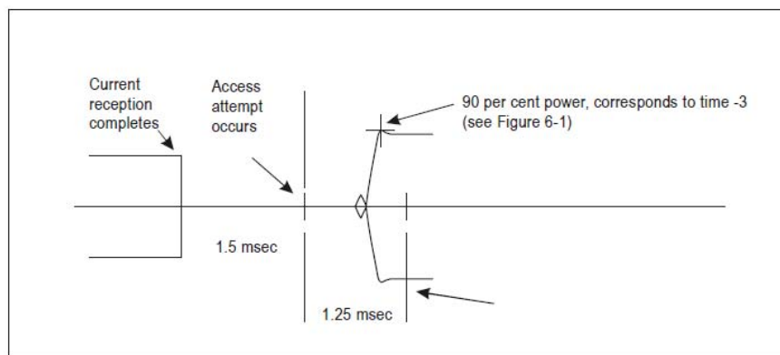
Figure 6-3. Receive to Transmit turnaround time
