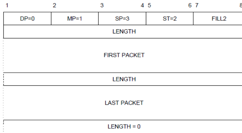
Figure 5-20. MULTIPLEX packet
