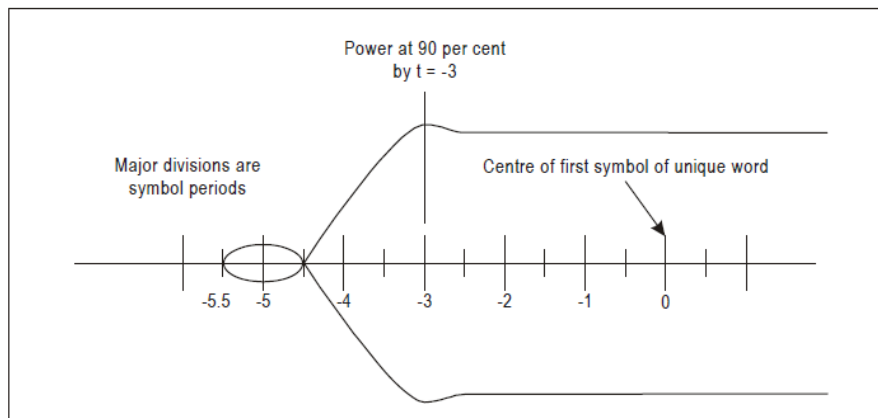
Figure 6-1. Transmitter power stabilization
