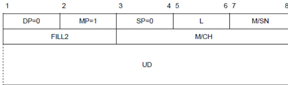
Figure 5-22. LONG FORM MSP packet
